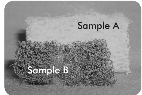
Samples A and B, shown above, were both taken from the same Full Cycle® floor pad. While Sample A was left untouched, Sample B was placed in an ASTM D5511 simulated landfill test for 290 days. Note the significant mass reduction via enhanced biodegradation in Sample B. Photo courtesy of Eden Labs LLC.
